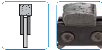
Standard 0.216" (5.5mm) high-output 'sandwich' segment designed to maintain profile during cutting
